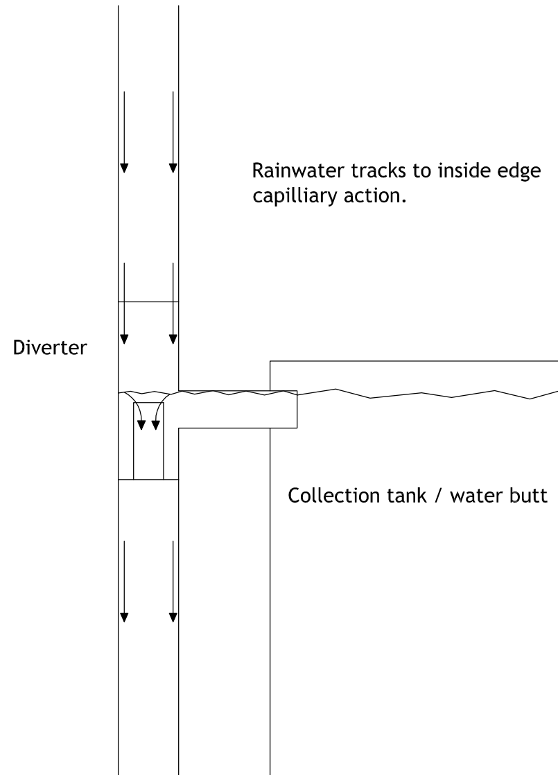
WORKING METHODOLOGY OF RAIN WATER DIVERTER - WHEN WATER COLLECTOR FULL
